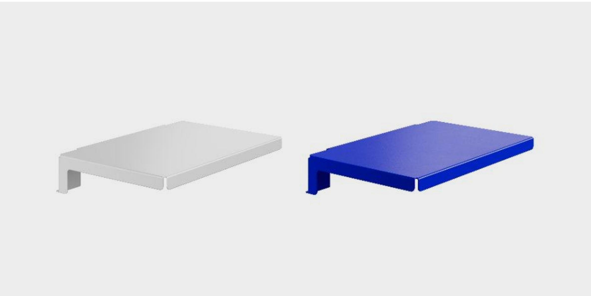
HANG ON Side Tray* Powder coated steel — W 330 x D230 x H65 mm
